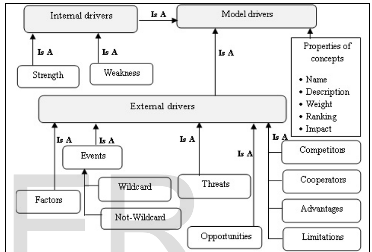
Fig.2. Conceptual model of Drivers KB
